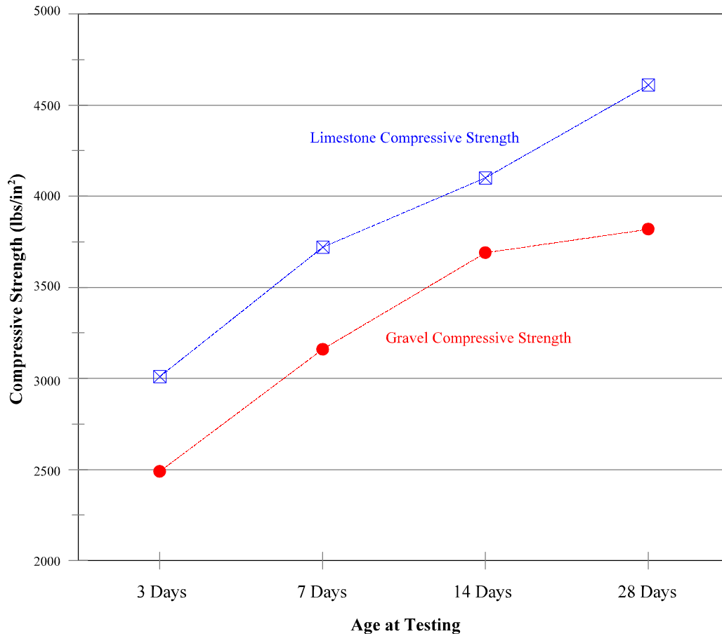
Graph 3 Compressive Strength
