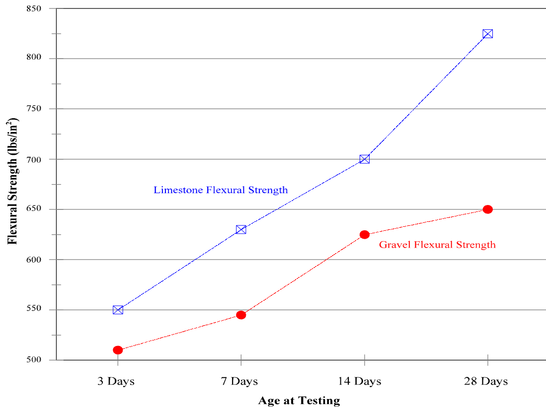
Graph 2 Flexural Strength
