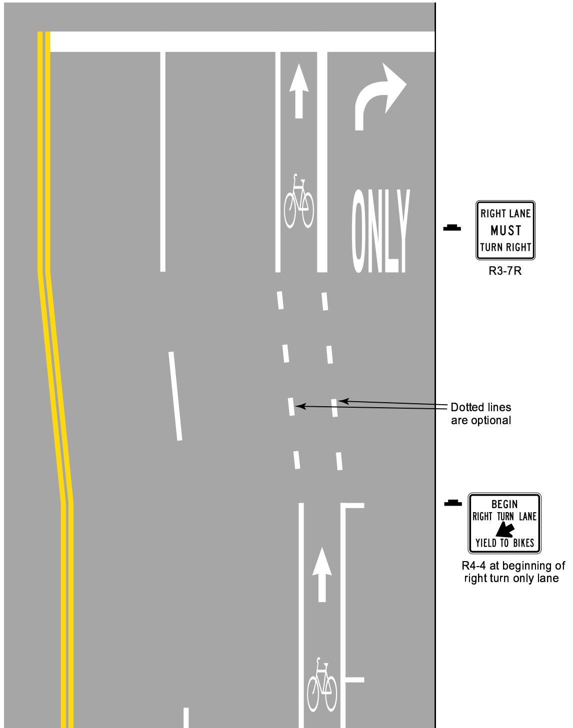
Figure 9C-4. Example of Bicycle Lane Treatment at Parking Lane into a Right Turn Only Lane
