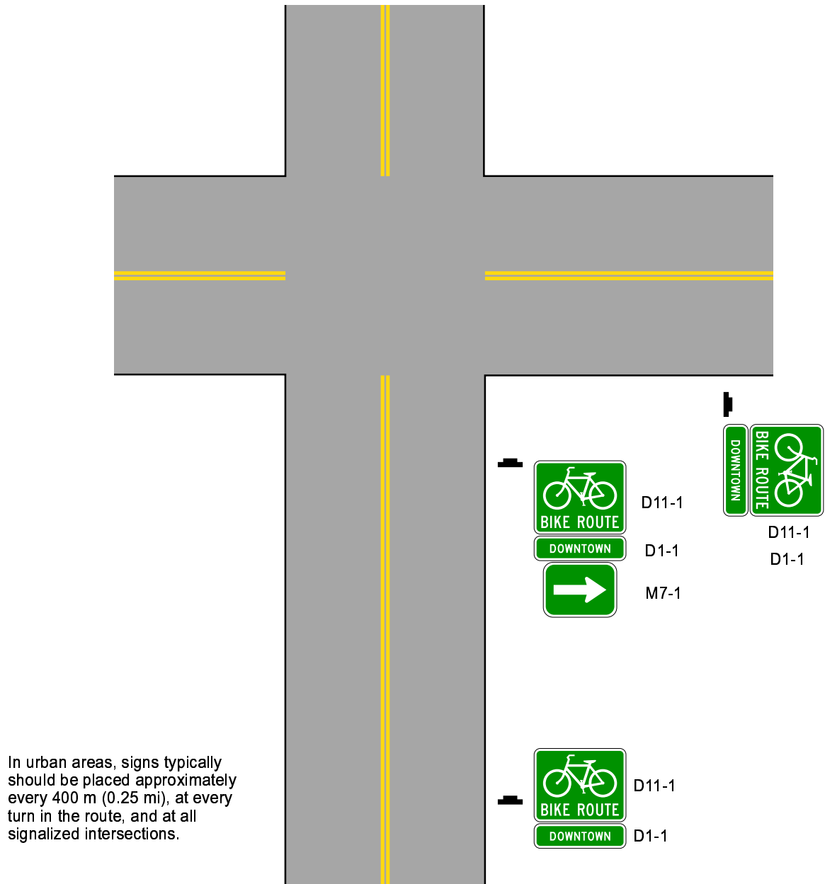
Figure 9B-6. Example of Signing for an On-Roadway Bicycle Route
