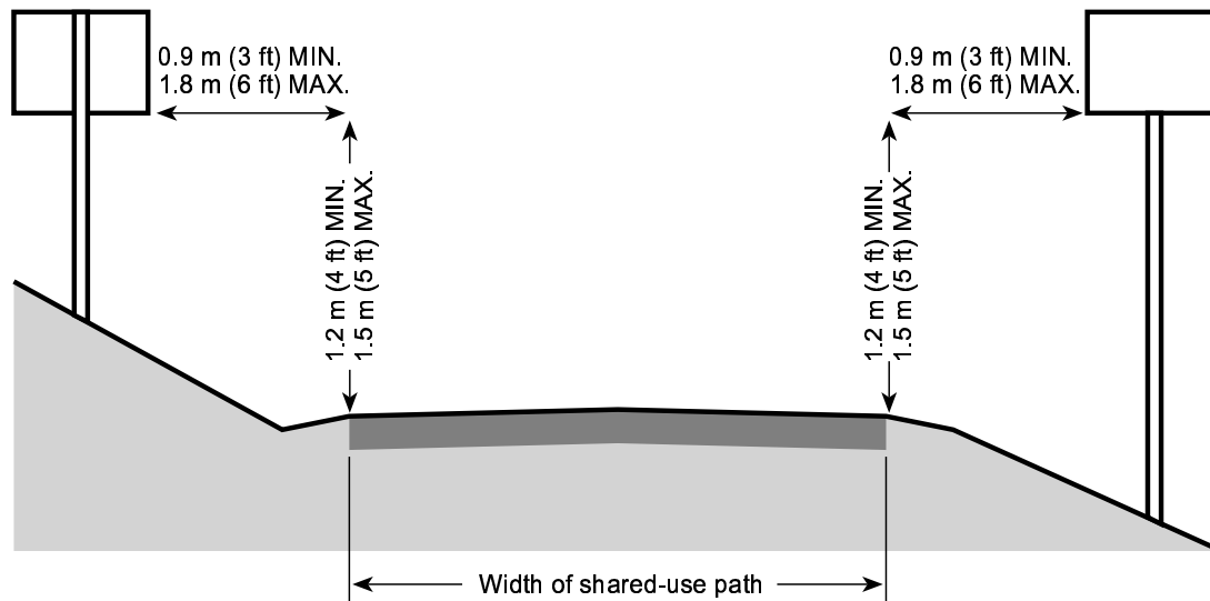
Figure 9B-1. Sign Placement on Shared-Use Paths
