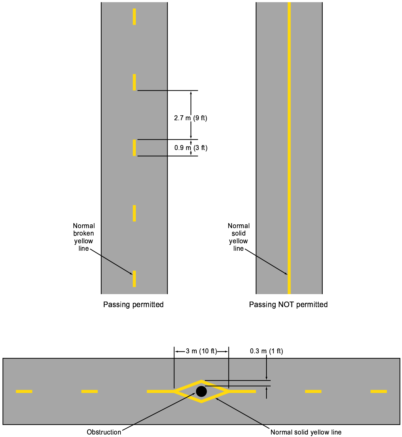
Figure 9C-2. Examples of Centerline Markings for Shared-Use Paths
