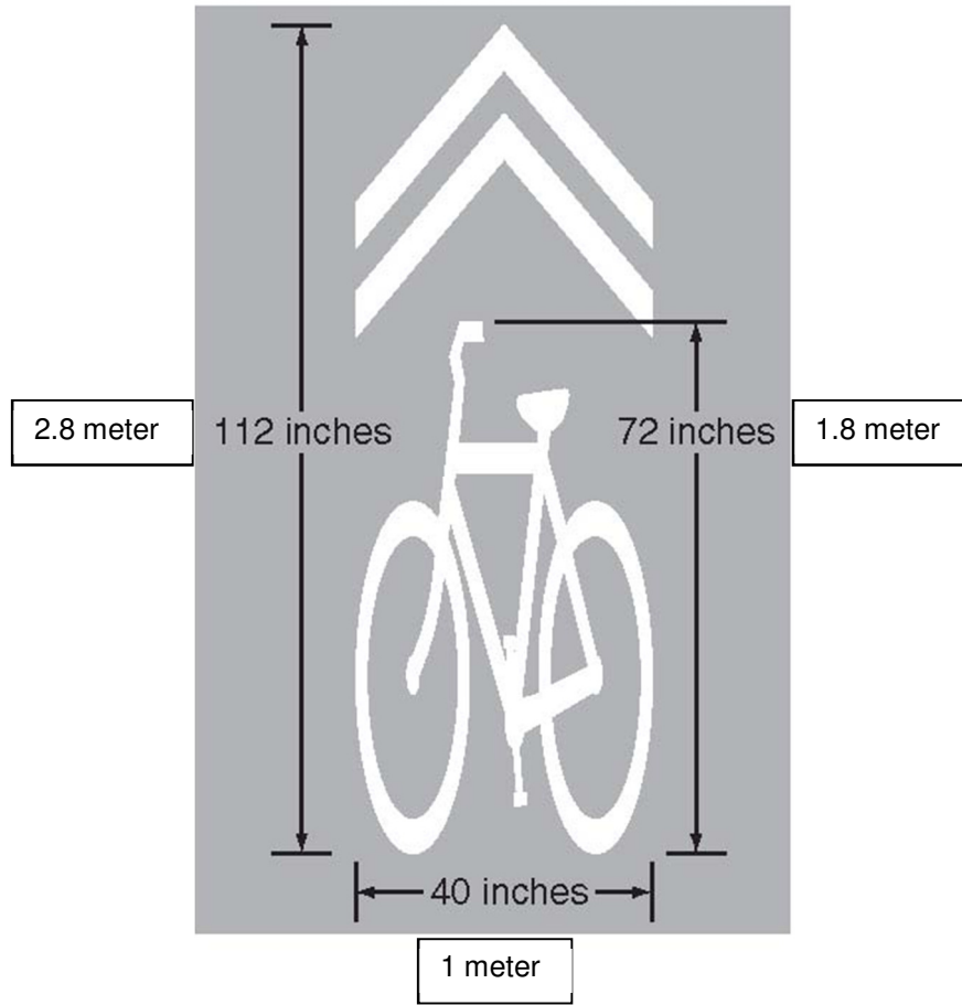
Figure 9C-9. Shared Lane Marking
