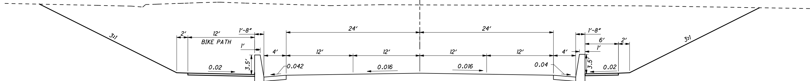
TYPICAL SECTION - 4 LANE SECTION WITH BARRIER AT RAILROAD BRIDGE
