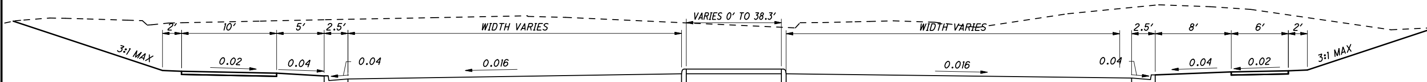
TYPICAL SECTION - SPLITTER ISLAND AT ROUNDABOUT
