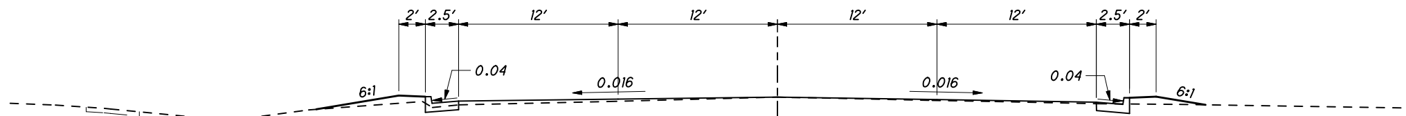
TYPICAL 4-LANE SECTION
