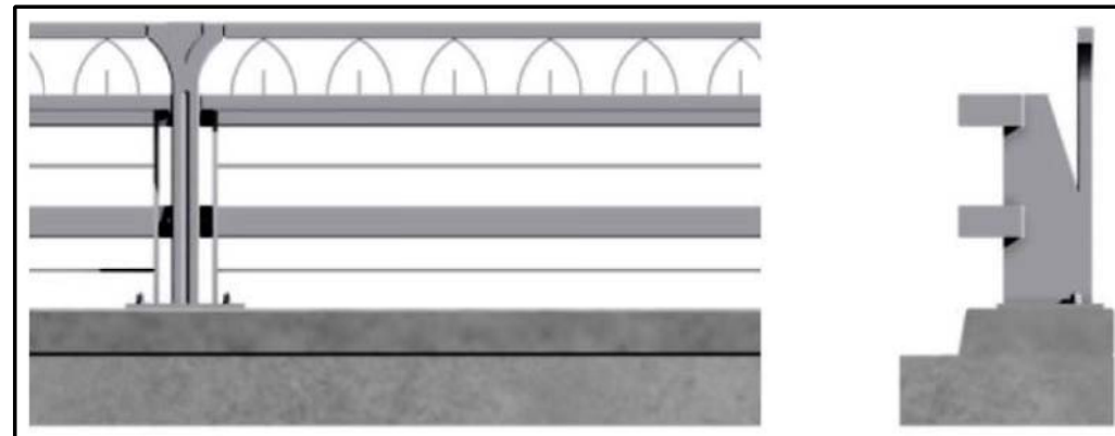
TRAFFIC/PEDESTRIAN COMBINATION BARRIER/RAIL CONCEPT
