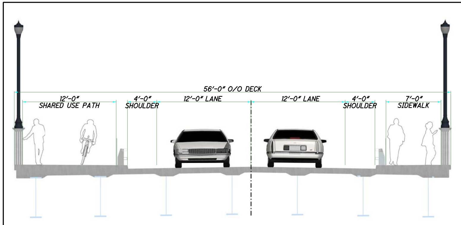
CROSS-SECTION
