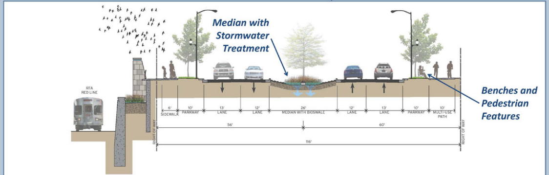
West and Central Sections: Typical Cross-Section Showing RTA
