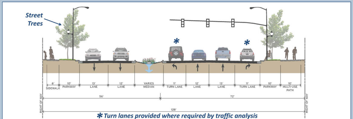
West and Central Sections: Typical Signalized Intersection Cross-Section
