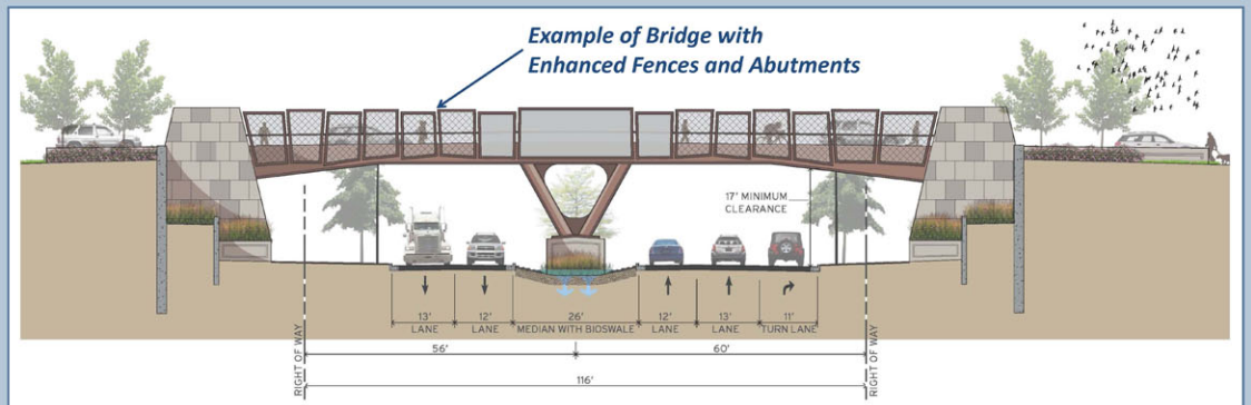
West and Central Sections: Typical Bridge Cross-Section
