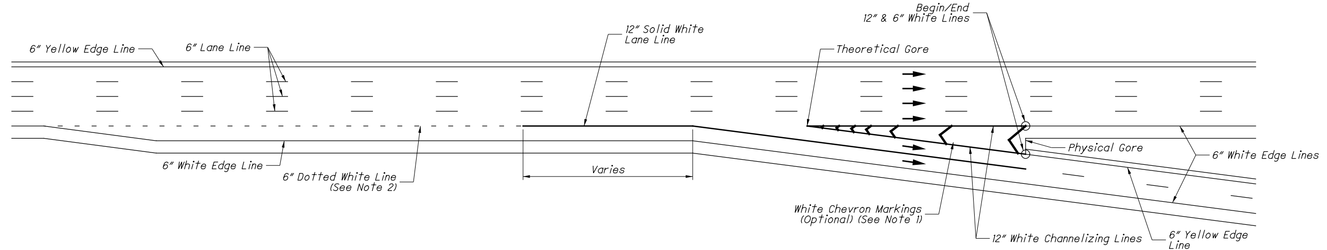
MULTI-LANE EXIT RAMP
