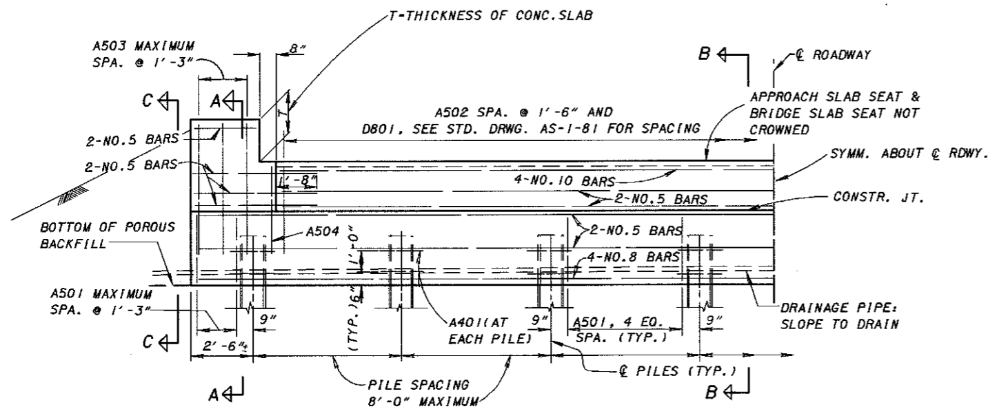
SEE SHEET [2/2] FOR SECTION C-C
