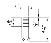
SINGLE THREADED INSERT (3,000 LB PROOF LOAD)
