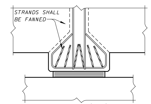
SECTION 12-12 (PARTIAL PIER AND DIAPHRAGM SHOWN)
