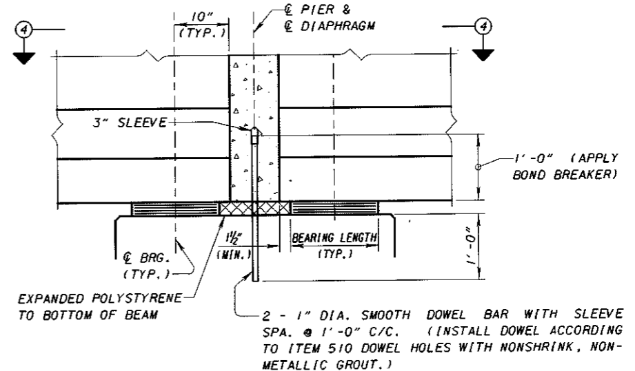
FIXED PIER DETAIL (BEARING WITH NO LOAD PLATE)
