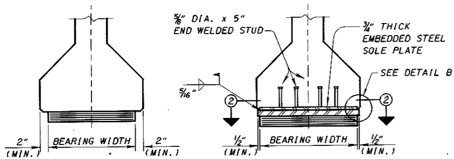
END VIEW (BEARING WITH NO LOAD PLATE)
