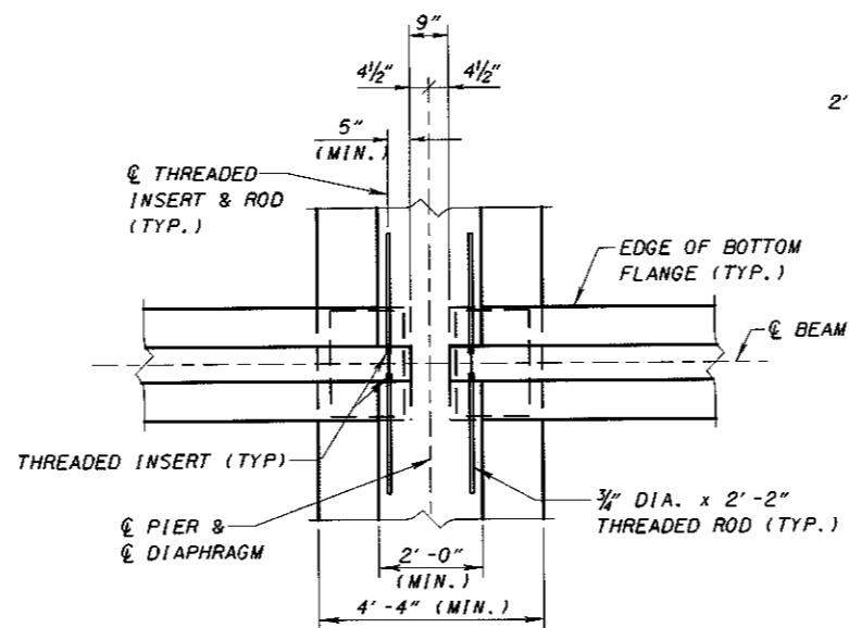
VIEW 3-3 (NO SKEW)
