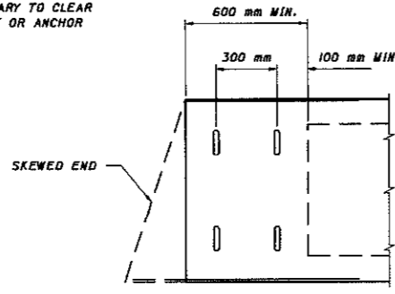
FOR 685 mm, 840 mm AND 1070 mm DEEP BEAMS
