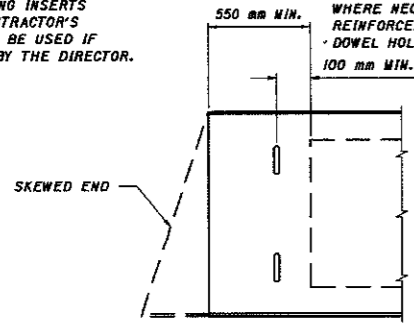
FOR 305 mm, 430 mm AND 535 mm DEEP BEAMS
