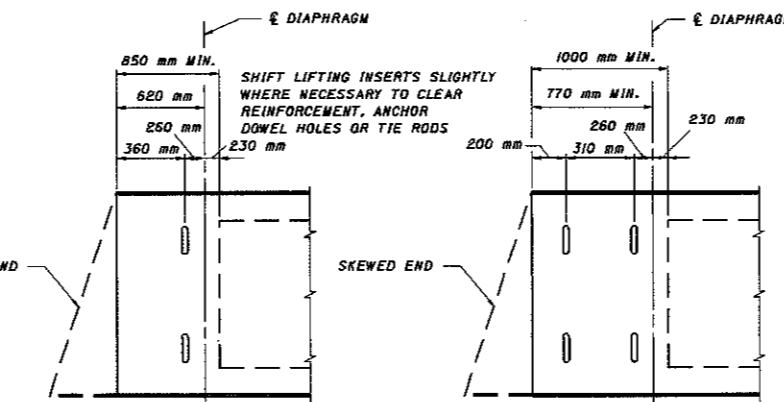
FOR 305 mm, 430 mm AND 535 mm DEEP BEAMS
