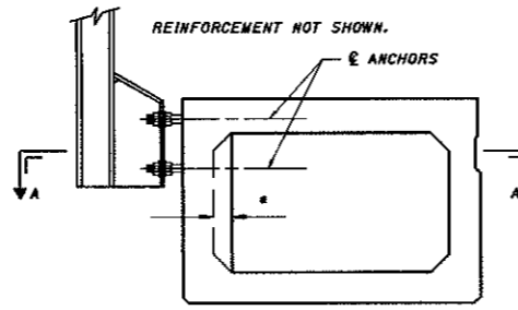
SECTION A-A SECTION SHOWING WALL THICKENING AT GUARDRAIL ANCHORS
