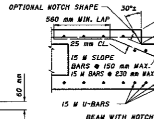
BEAM WITH NOTCH
