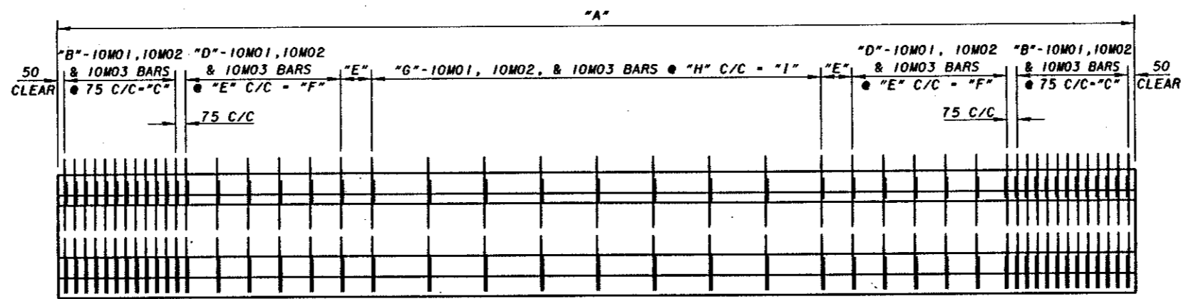
SHEAR REINFORCEMENT AASHTO TYPES 2, 3 & 4
