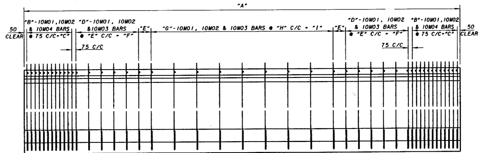
SHEAR REINFORCEMENT MODIFIED AASHTO TYPE 4 I-GIRDERS
