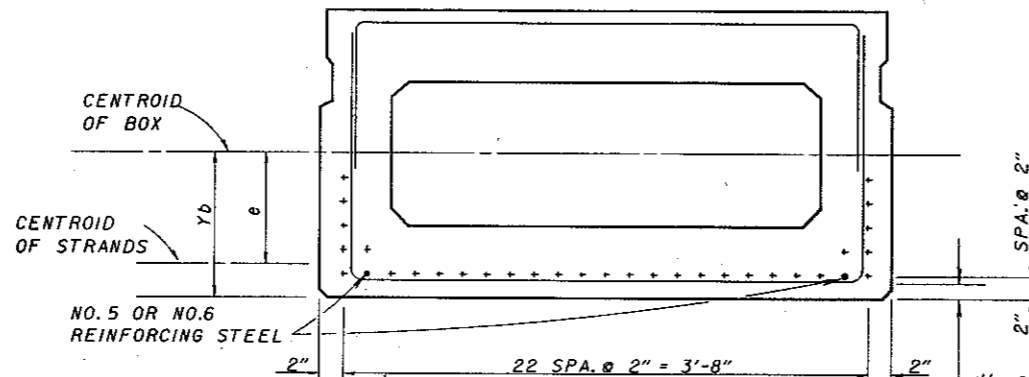
TYPICAL STRAND LOCATION
