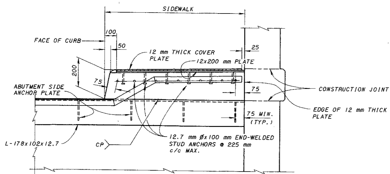
SECTION F-F
