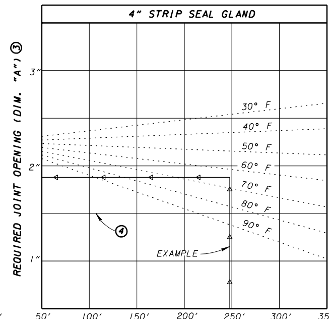
DISTANCE FOR DETERMINING JOINT OPENING ② TABLE C
