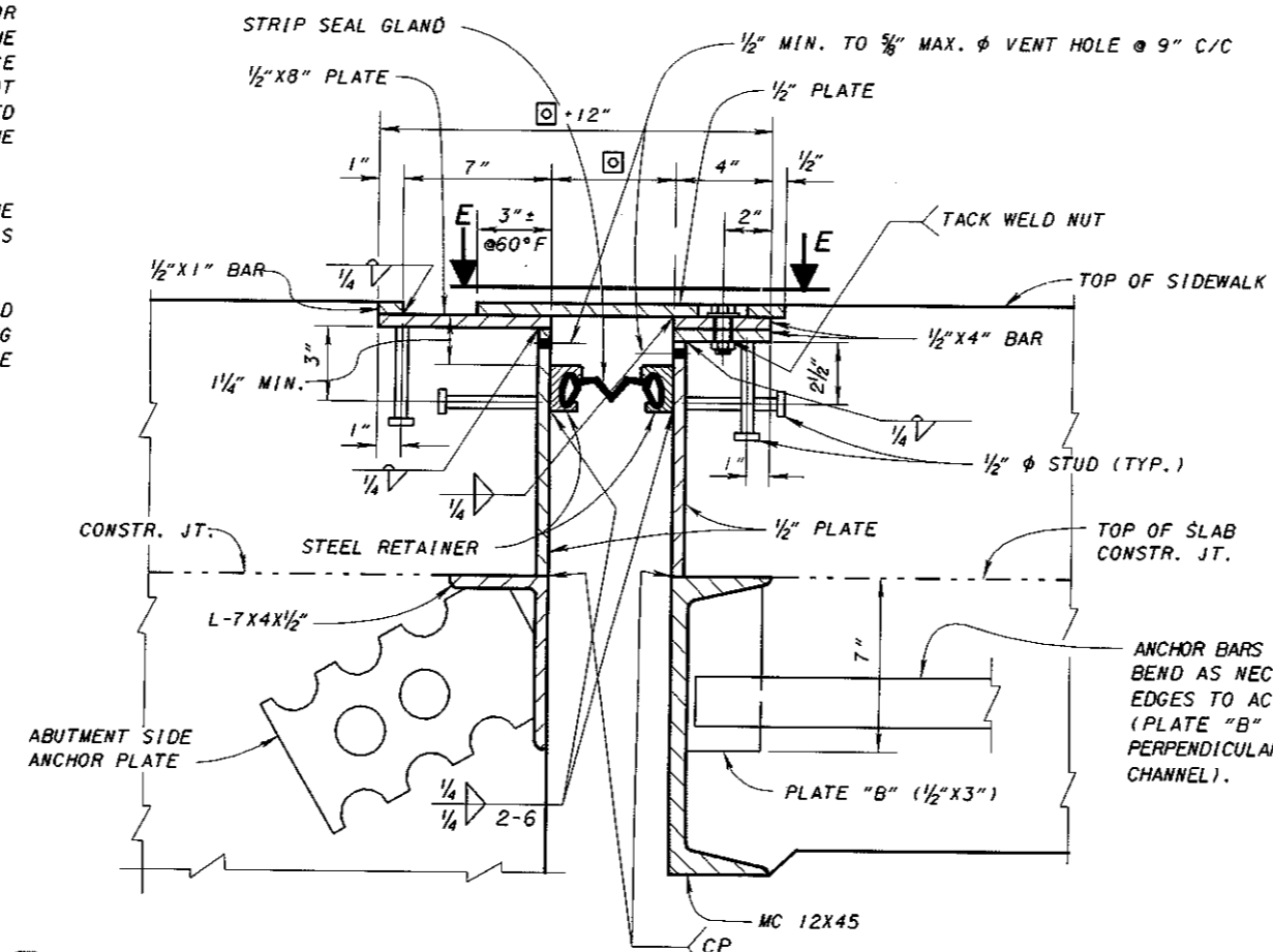
SECTION Y-Y
