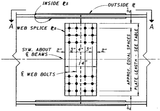
BEAM SPLICE DETAIL WEB SPLICE - TYPE A
