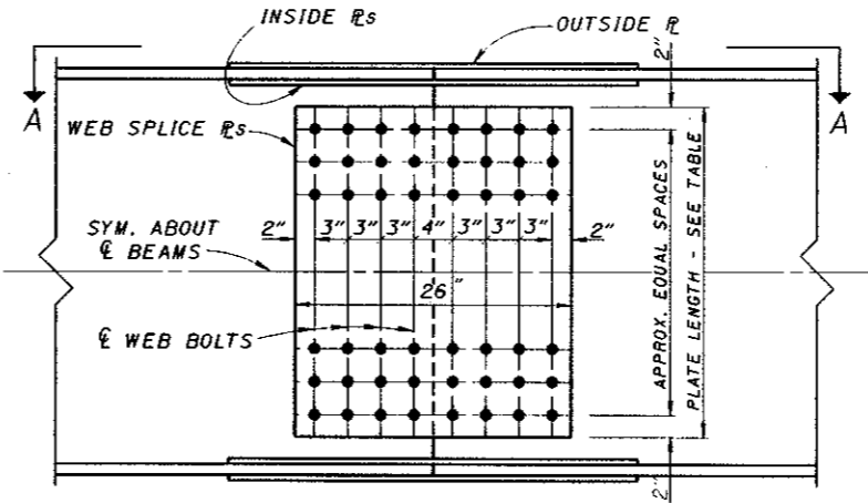
BEAM SPLICE DETAIL WEB SPLICE - TYPE C
