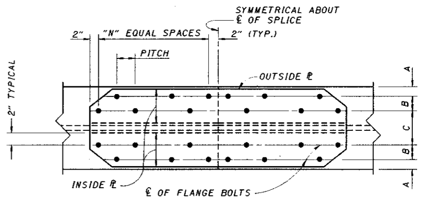
VIEW A-A FLANGE SPLICE - TYPE B
