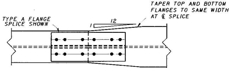
VIEW A-A SPLICE DETAIL FOR BEAMS HAVING DIFFERENT FLANGE WIDTHS
