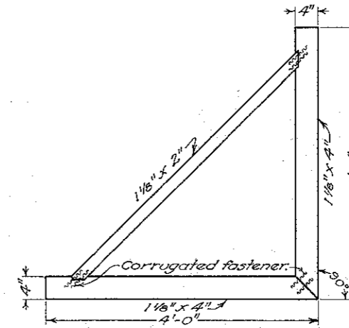
SQUARE FOR SETTING TRANSVERSE JOINTS
