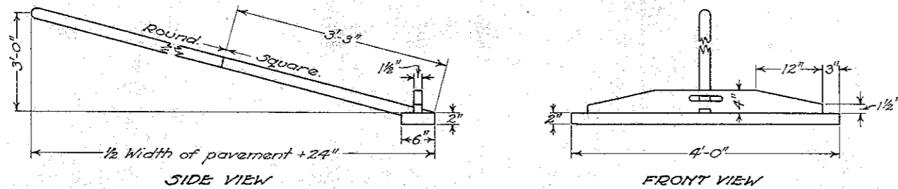
LIGHT SMOOTHING LUTE
