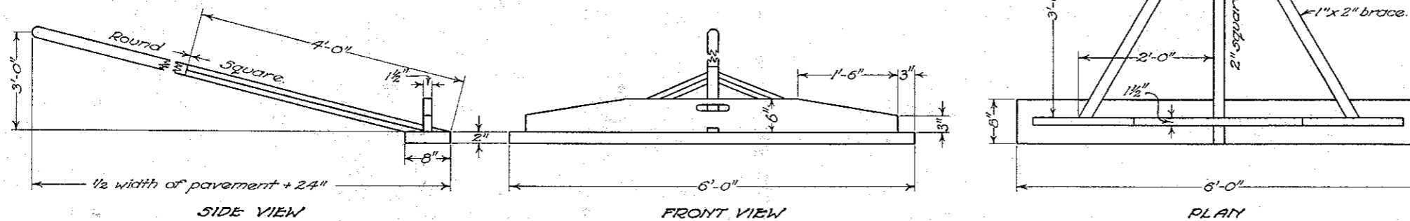
HEAVY SMOOTHING LUTE
