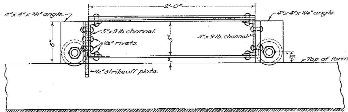
SECTION A-A (ENLARGED)
