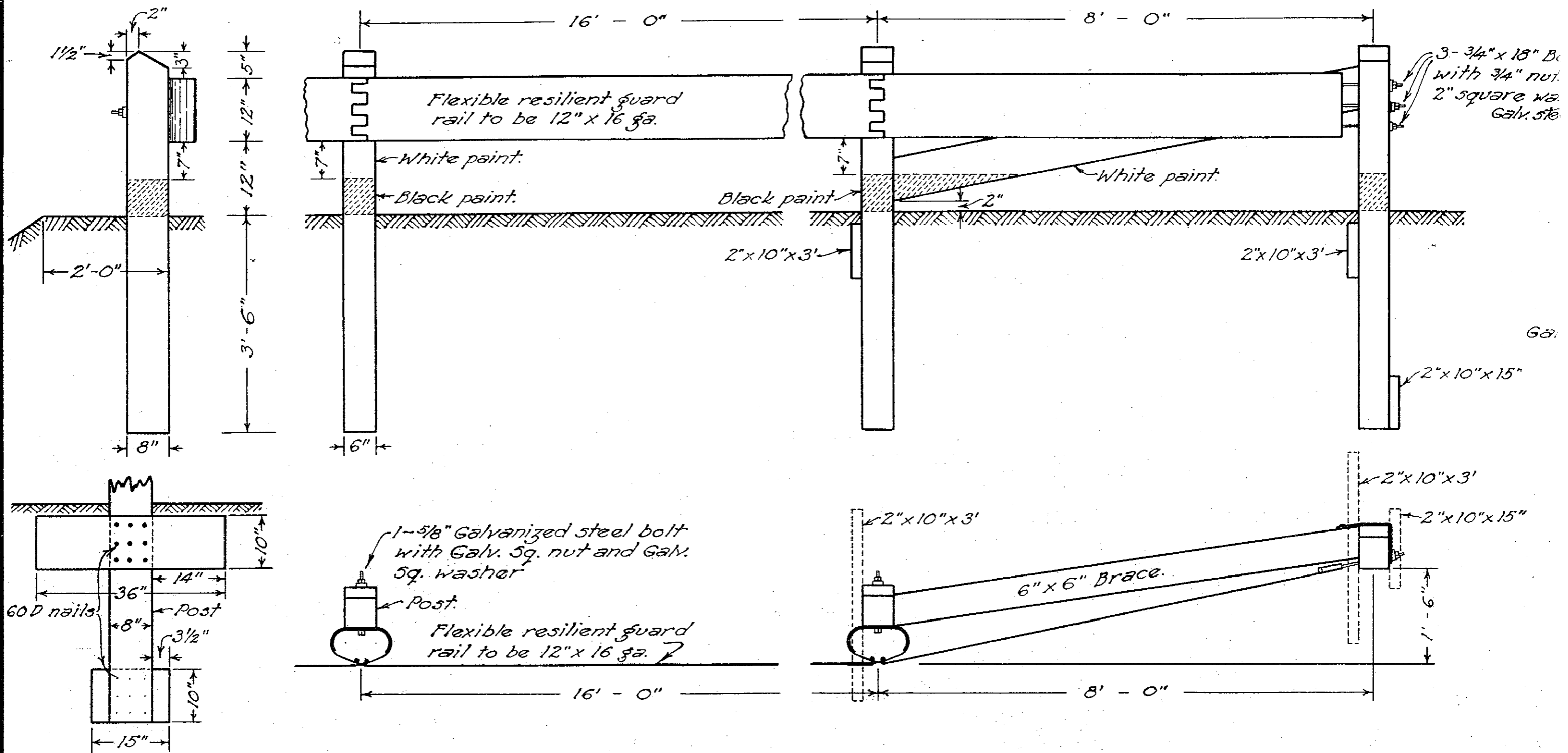
DETAIL SHOWING ATTACHMENT OF ANCHOR TO POST
